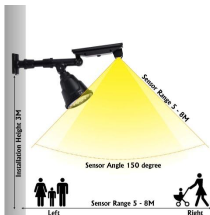
Wall punching install way
